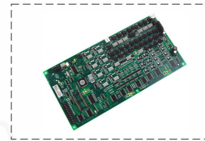
MF3/MF3-C/MF3-S Tke elevator pcb board
