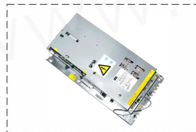
KDL16R Kone elevator inverter
