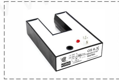
KM86420G03 Kone leveling sensor
