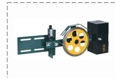
OX-200 Elevator Tension Device
