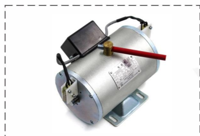
DZS800AB01D1 Xinda elevator brake
