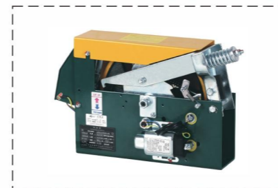
OX-240A Elevator governor
