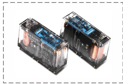
G7SA-3A1B Omron salay relay
