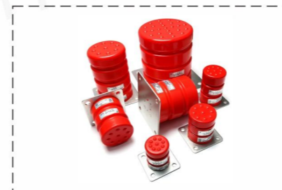
LD-HC-L1/L2/L3-25 Elevator polyurethane buffer
