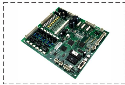
LCB-II Xizi otis main board
